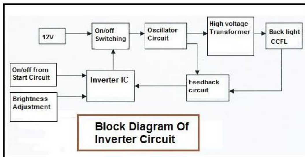
Block diagram of Buck Royer inverter
